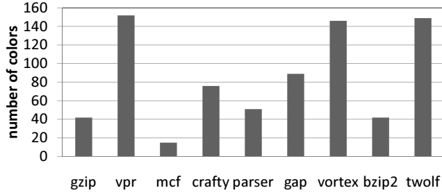
Figure 4. Number of colors for SPEC benchmarks.
