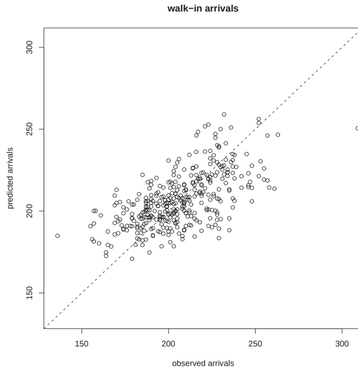
Figure 2.2: Example scatterplot.
