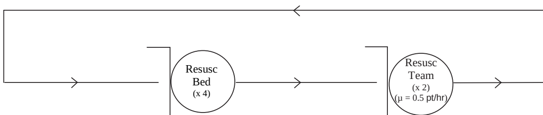
Figure 5.2: Lower-levels of closed queueing network model of patient flow.
