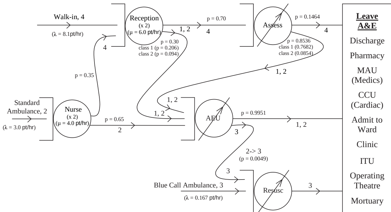
Figure 4.2: Top-level of queueing network model of patient flow.
