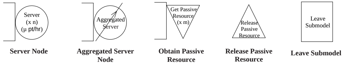
Figure 4.1: Queueing network model notation.
