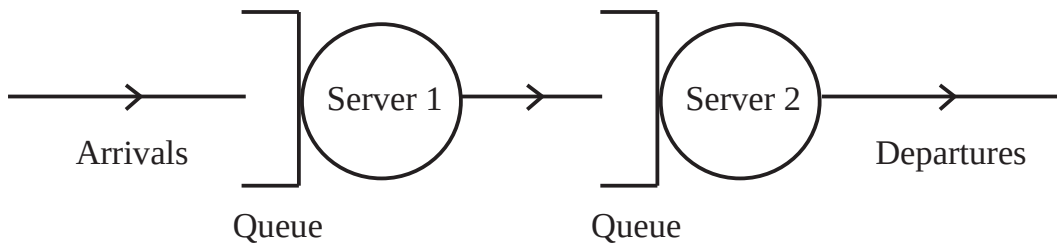
Figure 2.3: Example queueing network.
