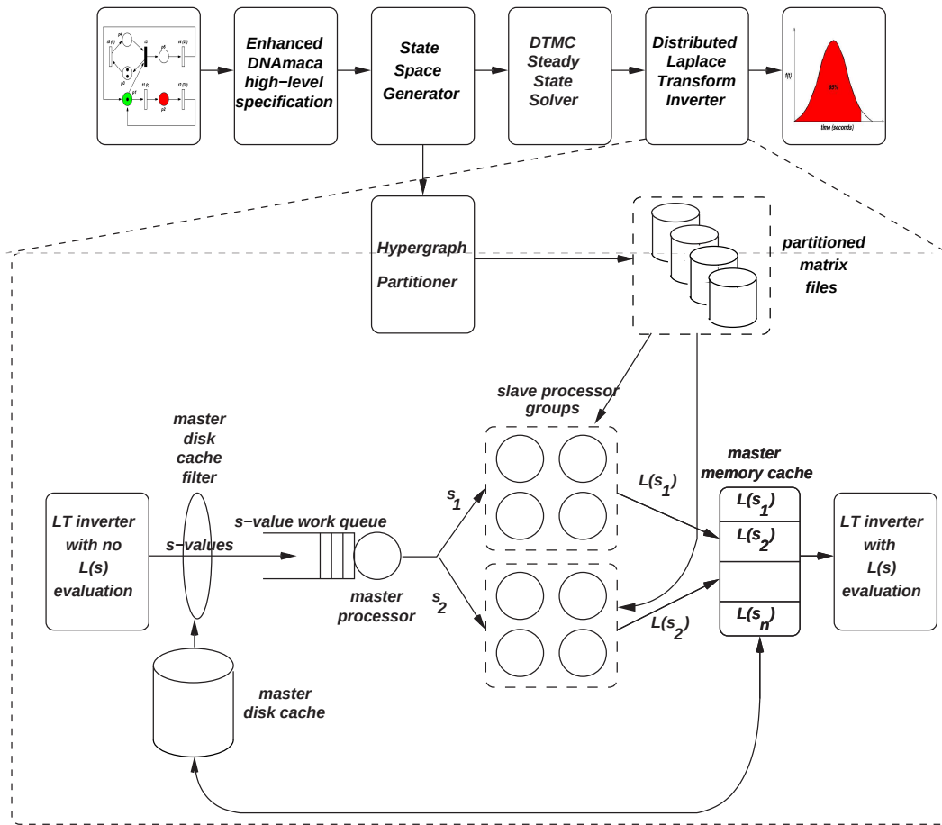
Figure 2.5: Passage time analysis pipeline.
